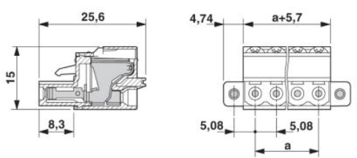
Dimensioned drawing
