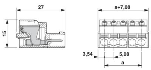
Dimensioned drawing
