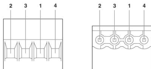
Pin assignment left
