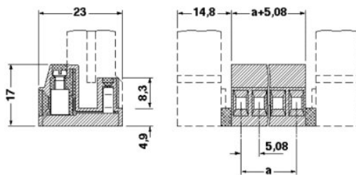
Dimensioned drawing
