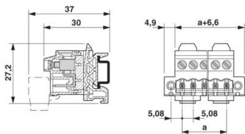
Dimensioned drawing
