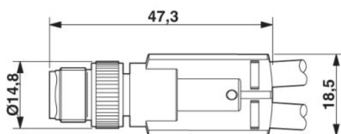
Plug M12 x 1, Y distributor
