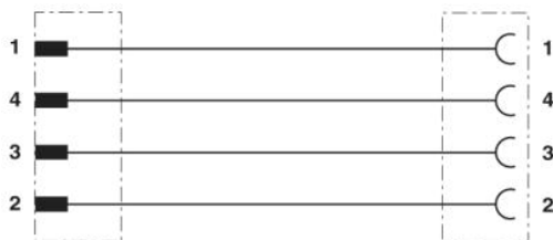
Contact assignment of M12 plugs / M8 sockets
