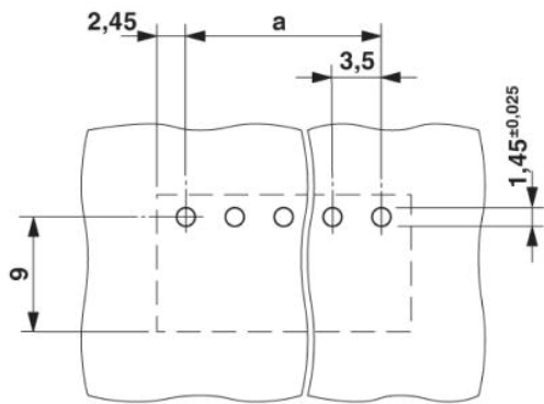
Dimensioned drawing
