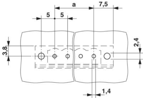
Drilling diagram
