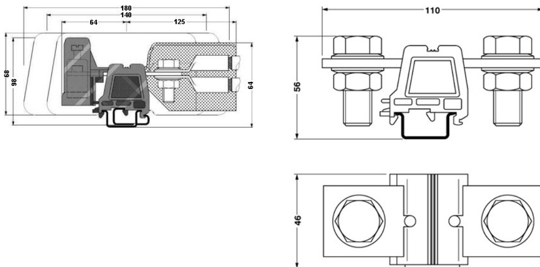
Dimensioned drawing
