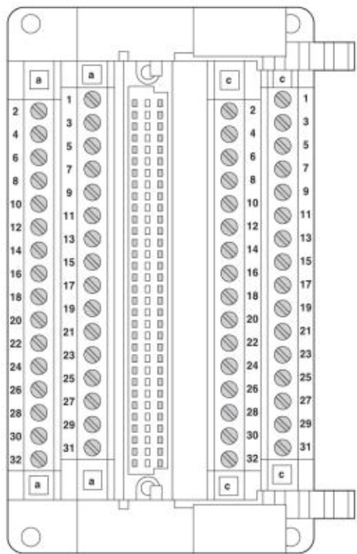
Schematic diagram
