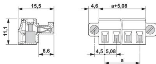
Dimensioned drawing
