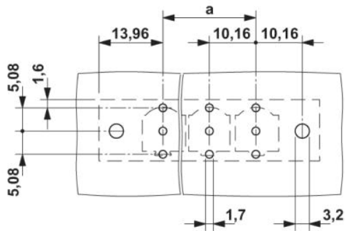
Drilling diagram
