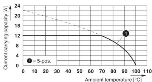
Derating curve for: TFKC 2,5/..-STF-5,08 AU with CC 2,5/..-GF-5,08 P26THR AU
