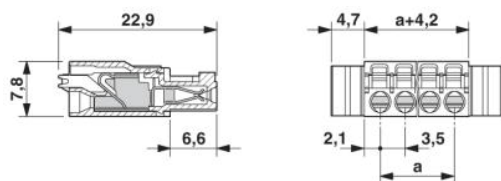
Dimensioned drawing
