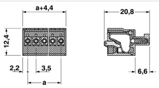
Dimensioned drawing
