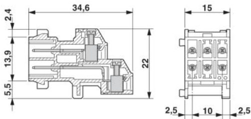
Dimensioned drawing
