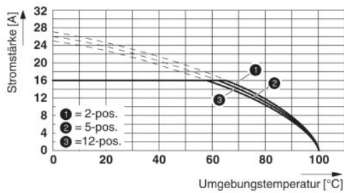
Derating curve for: GIC 2,5 HCV/...-ST-7,62 with GIC 2,5 HC/...-G-7,62
