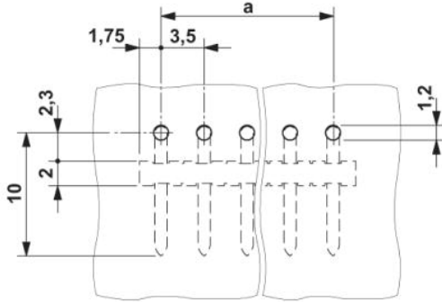
Drilling diagram
