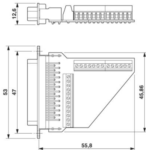
D-SUB contact insert
