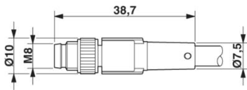
M8 x 1 male connector, straight version
