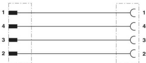
Contact assignment of M8 plugs/sockets
