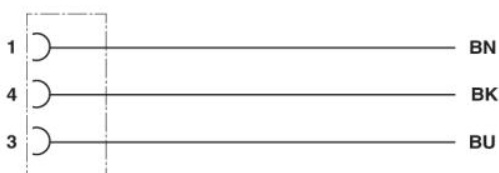
Contact assignment of M8 socket
