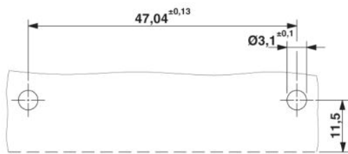
Drilling diagram
