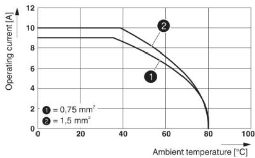
Derating diagram: A series
