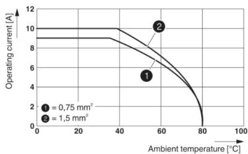
Derating diagram: HC-A3...Q1,5...
