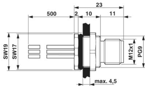
M12 flush-type plug
