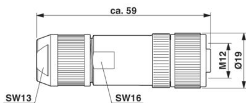
M12 x 1 female connector, straight, shielded
