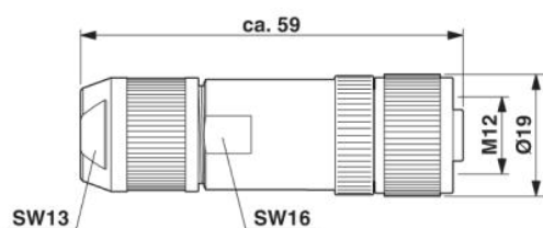
M12 x 1 female connector, straight
