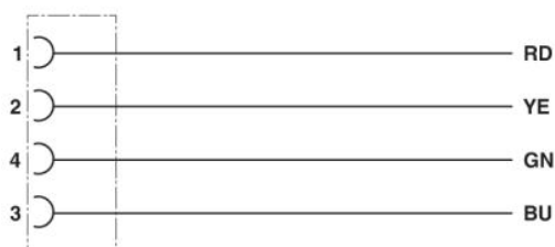
Contact assignment of M8 socket
