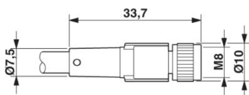
M8 x 1 female connector, straight version
