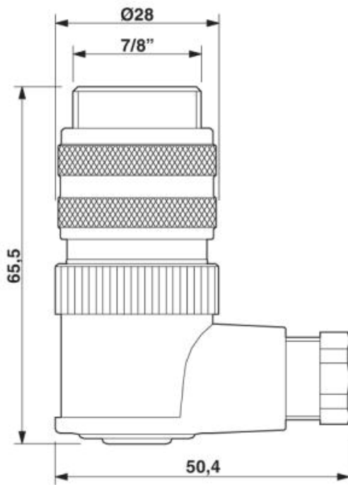
Dimensioned drawing
