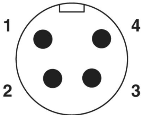
Schematic diagram
