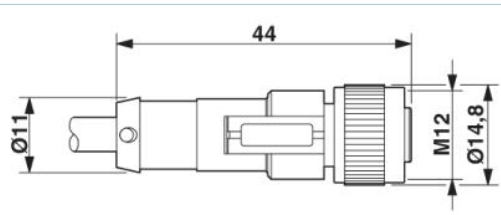
M12 x 1 female connector, straight
