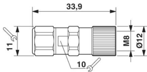
Dimensioned drawing
