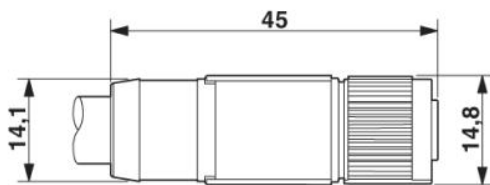
Socket M12-SPEEDCON, straight, shielded
