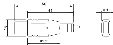
Dimensional drawing
