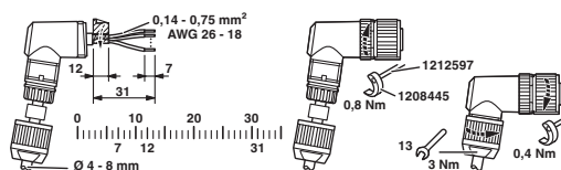
Functional drawing
