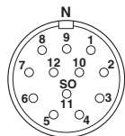
Connector pin assignment
