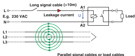
Application drawing
