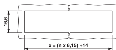
Dimensional drawing
