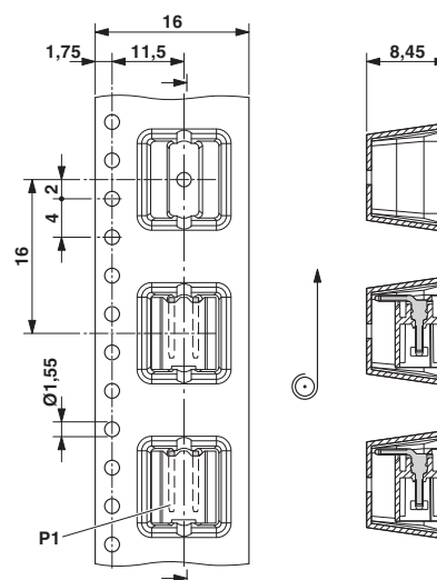
Dimensional drawing
