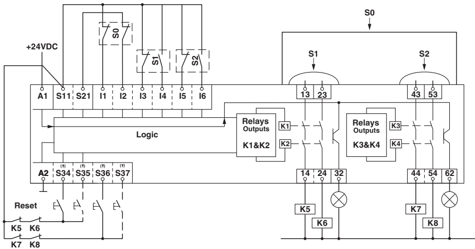
Circuit diagram
