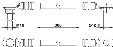
Dimensional drawing
