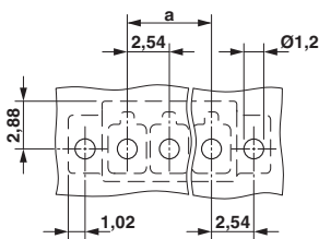
Drilling diagram
