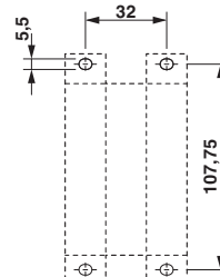
Dimensional drawing
