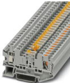
Knife disconnect terminal block, connection method: Push-in connection, Screw connection, cross section: 0.2 mm 2 - 6 mm 2 , AWG: 24 - 12, width: 6.2 mm, color: gray, mounting: NS 35/7,5, NS 35/15
