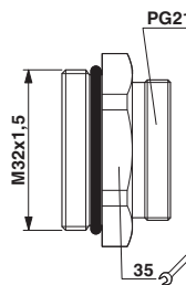
Dimensional drawing
