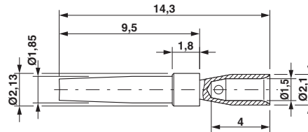
Dimensional drawing
