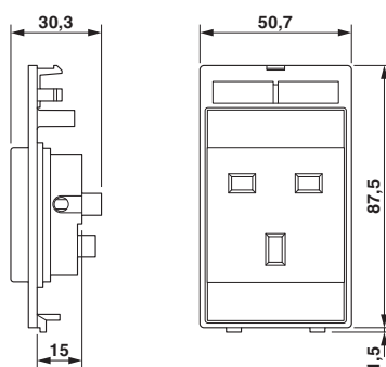
Dimensional drawing
