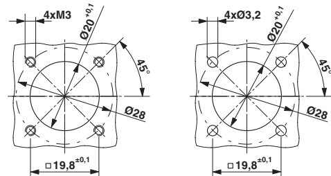
Installation dimensions
