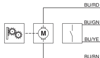
Block diagram of the locking actuator
